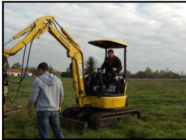
Installation de poteaux
